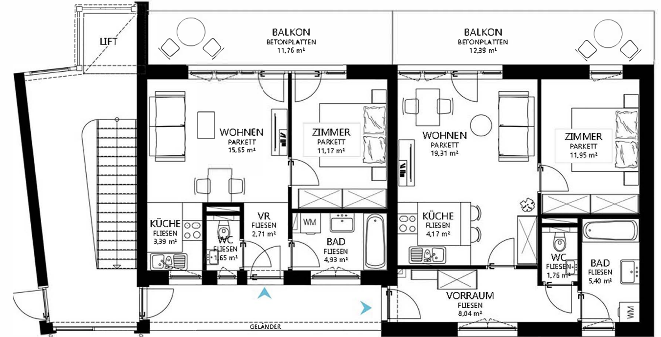
WFL 39,50 m 2 TOP 37 & 41
